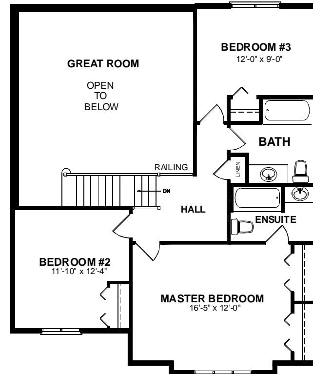
SECOND FLOOR PLAN 772 SQ. FT.
